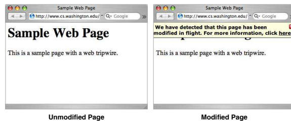
Figure 2: If a web tripwire detects a change, it displays a message to the user, as in the screenshot on the right.
