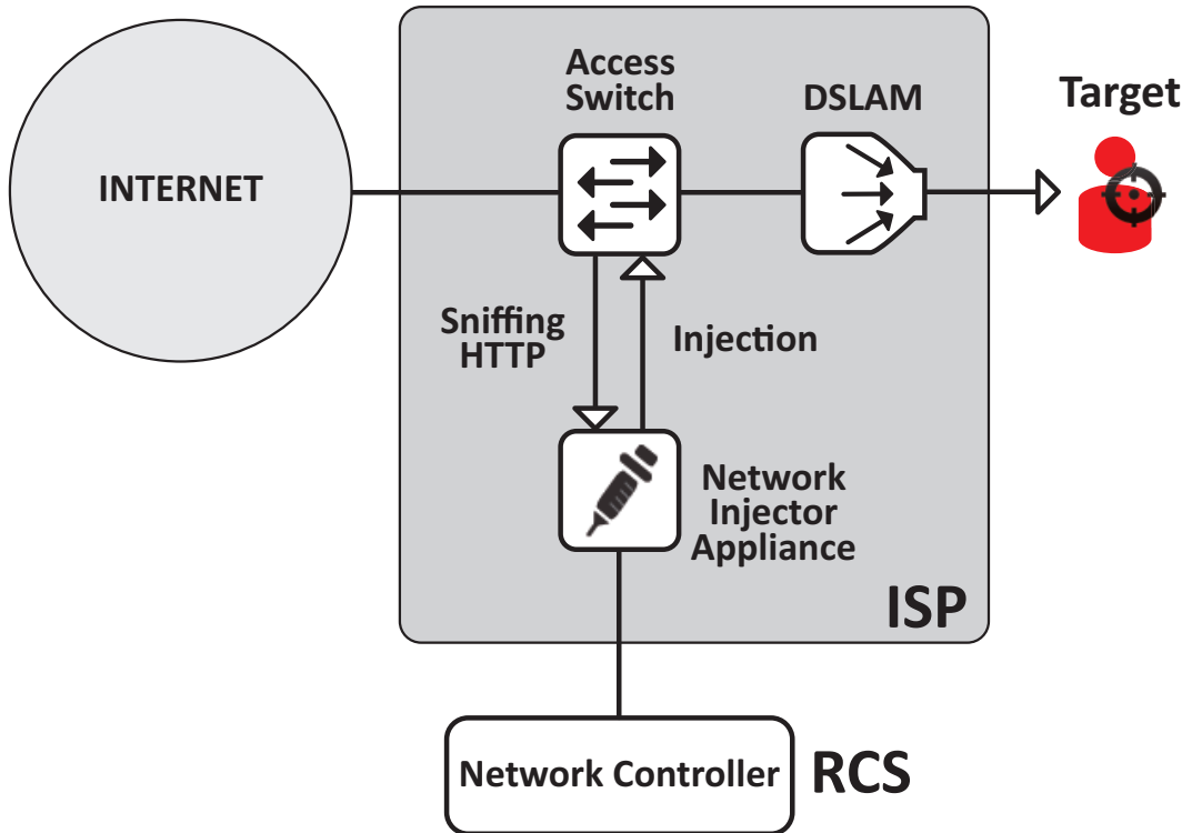
Figura 1: Network Injector Appliance: schema fisico
