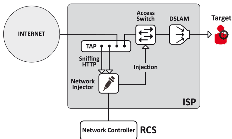
Figura 2: Network Injector Appliance with TAP: physical layout
