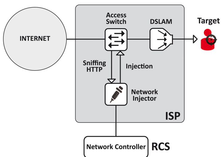
Figura 1: Network Injector Appliance in LAN: physical layout
