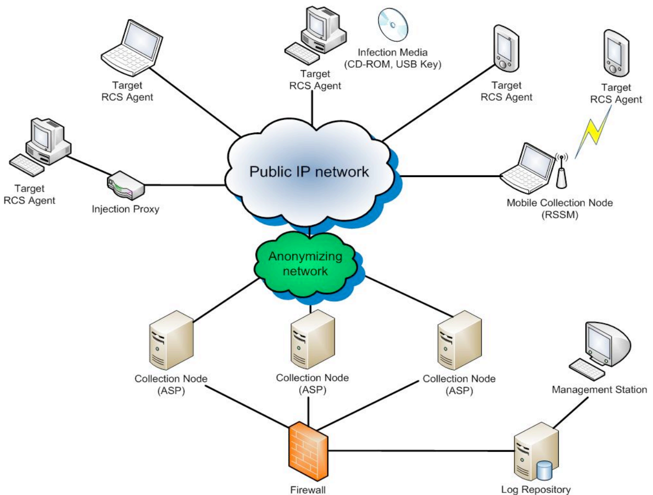
RCS Aschitecture
