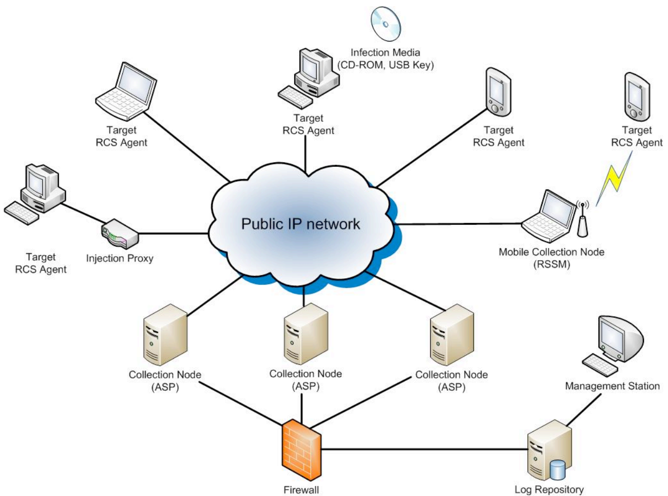
RCS Aschitecture
