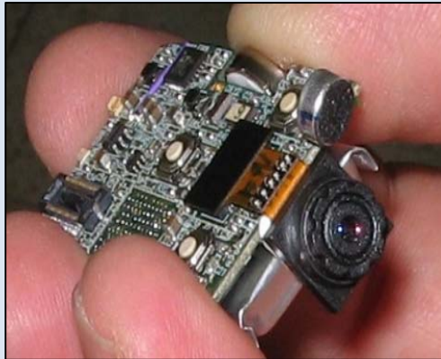
5610 - New Video/Audio Digital Recorder
