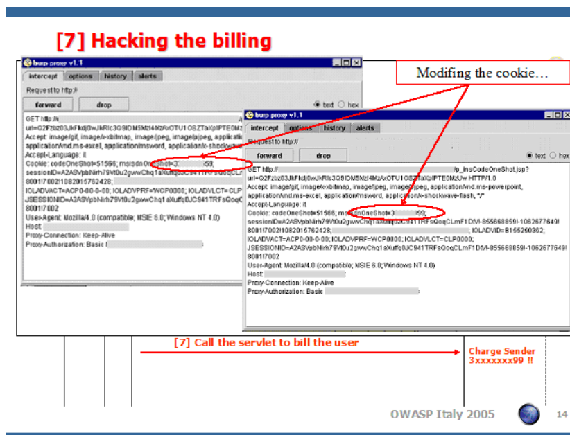
Example of Cookie with identity in clear text
