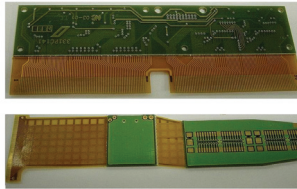
RF Mix Pcb Rogers to Fr4
