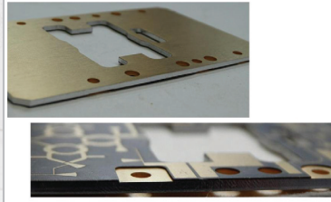
Rogers 5880 and alluminium with some milling depth control
