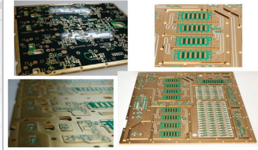
RF- 10 layers RO4350b and copper clad 5mm inside
