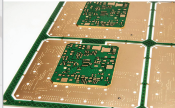
Flex-Rigid pure gold 99,99 % 2 \mu to 8 \mu
